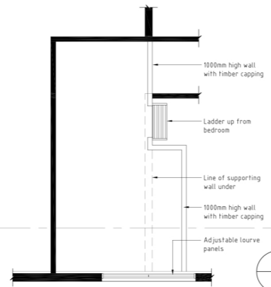
2 MEZZANINE PLAN 1:50 @ A1, 1:100 @ A3
